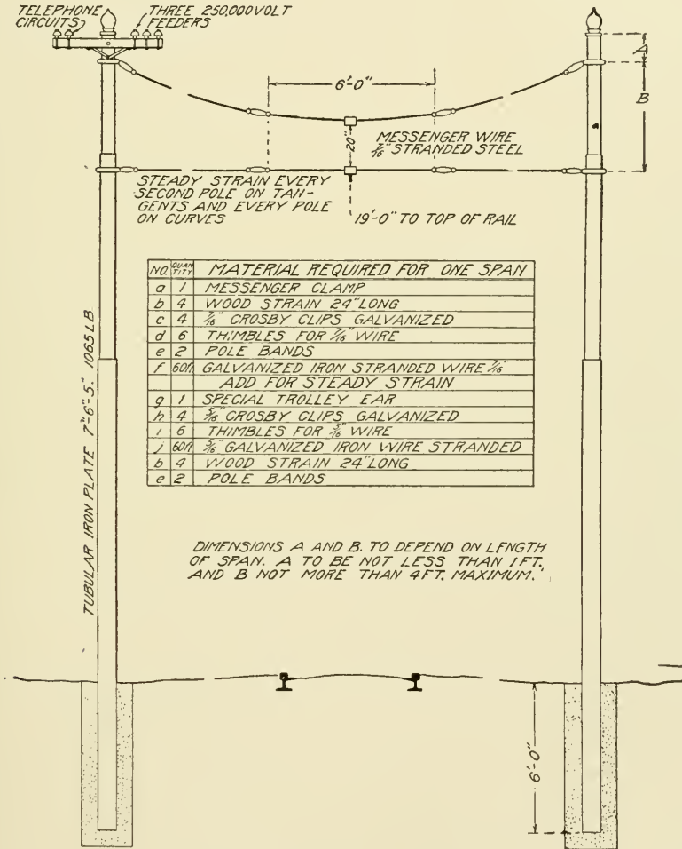
Fig. 198. Span Construction of the Catenary Type
